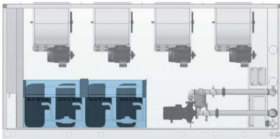
2 Pumps configuration (NECS-C 4 compressors)
